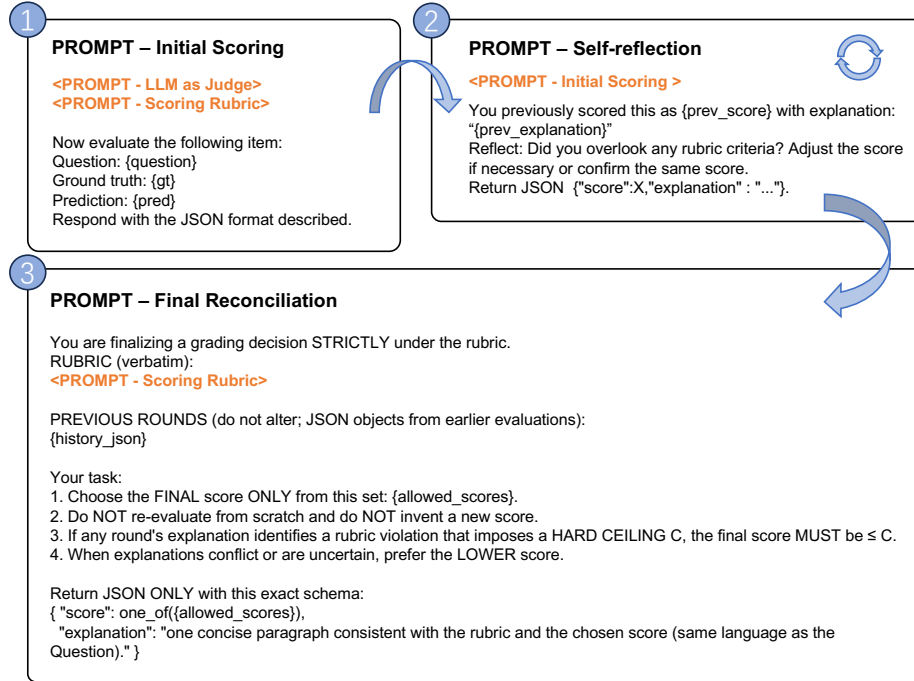
Fig. 9: CoT LLM-as-a-Judge prompts. Overview of the three prompts used in SCORING-REFINE: (1) Initial Scoring, which grades a prediction against the ground truth under the rubric; (2) Self-reflection, which revisits the previous score and explanation; and (3) Final Reconciliation, which aggregates all rounds and outputs the final score and explanation.
